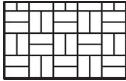
Basket Weave Brick Size 200 x 90mm
